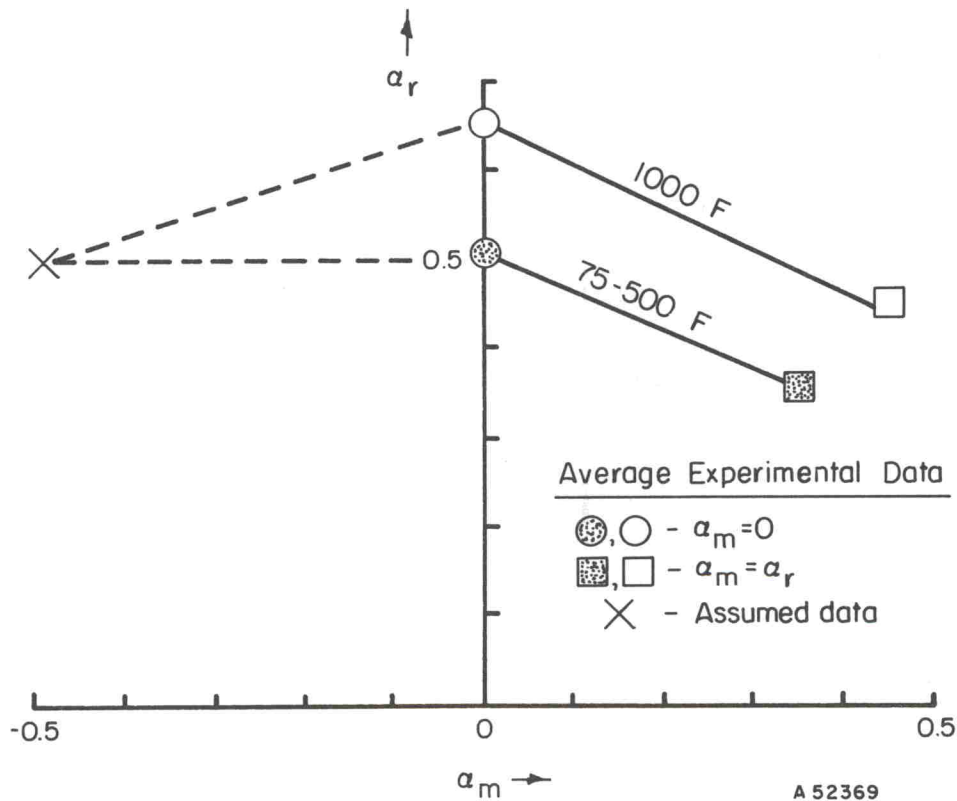
FIGURE 42. FATIGUE DIAGRAM FOR 10^4 - 10^5 CYCLES LIFE FOR HIGH-STRENGTH STEELS AT TEMPERATURES OF 75 F TO 1000 F \alpha_r and \alpha_m are defined by Equations (10a, b)
